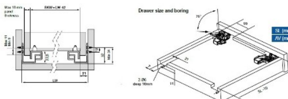
Drawer size and boring
